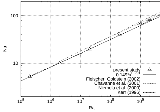
Figure 1. Comparison of the computed Nu(Ra) results with several experimental and DNS correlations.
