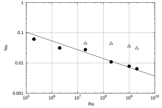
Figure 2. Viscous ( \triangle ) and thermal ( \bullet ) boundary layer thicknesses vs Ra . Line is power law \delta \sim Ra^{-0.291} .
