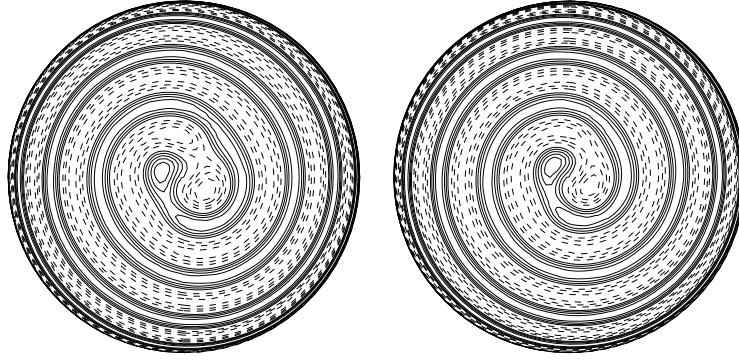
Figure 1. Contours of radial flow u_r at the middle surface of the spherical shell for \epsilon = (R/R_c) - 1 = 0.28 ( R_c = 1712 ) and Pr = 7.0 . Dashed contours indicate radially inward flow u_r < 0 and solid contours correspond to radially outward flow u_r > 0 . The top (middle) panel shows the contours viewed from the north (south) pole.
