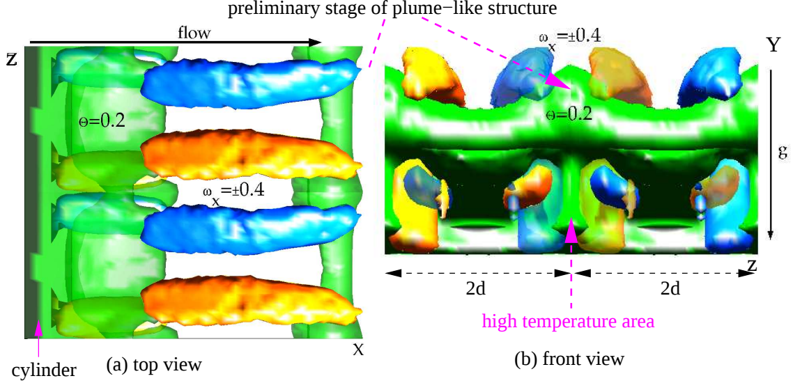
Figure 2: Snap-shot of calculated iso-vorticity \omega_x = \pm 0.4 surfaces and iso-temperature \Theta = 0.2 surface at Ri = 1.0 , Re = 85 . The spanwise distance of the streamwise-vortices-pair is around 2d , d is the cylinder diameters.
