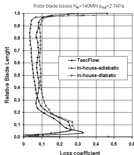
Fig.2. Loss coefficient distributions along the blade length
