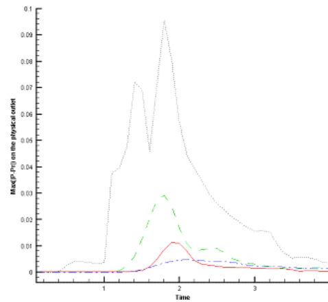
Figure 2. Time history of the maximum error in pressure fluctuations at outlet. —, NSPML (10 grids); --- Freund's buffer zone (10 grids); - · - · -, Freund's buffer zone (40 grids); ·····, NSCBC.
