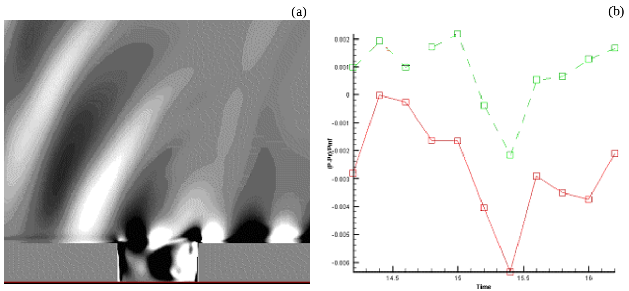
Figure 3. Computation of open cavity flow with NSPML. (a) Pressure wave; (b) time history of pressure error at the mid-point of domain outlet; —□—□—, NSPML; - □ - □ -, Freund's buffer zone.
