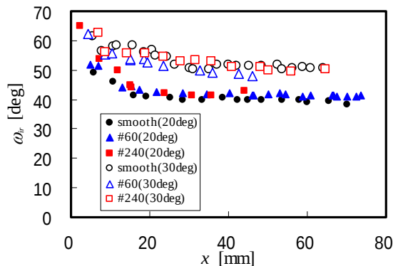
Fig. 3 The angle \omega_{ir} between incident and reflected shocks
