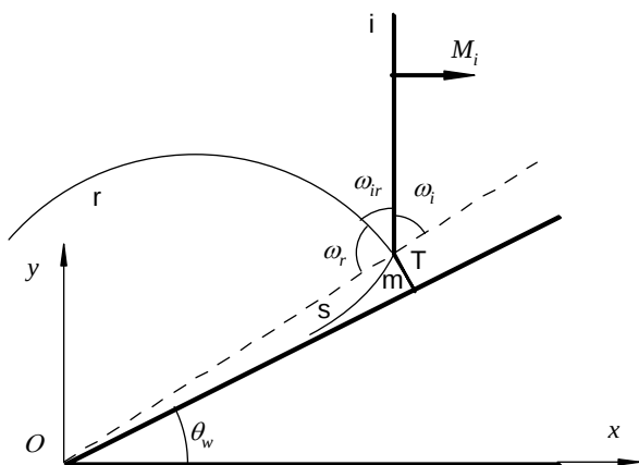
Fig. 1 Definition of geometric variables
