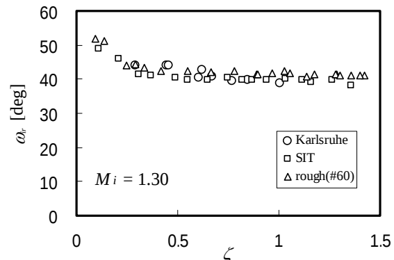
Fig. 4 The angle \omega_{ir} in the dimensionless coordinate
