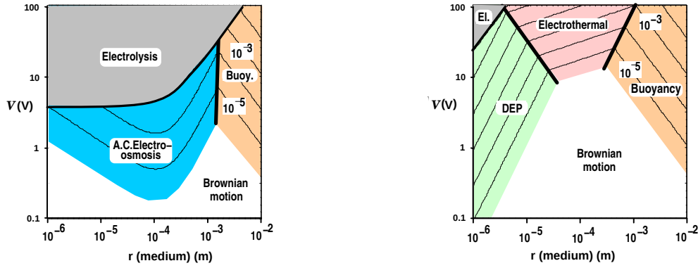
Figure 1. Particle velocity maps in the plane V versus r for a particle with radius a = 0.25\mu\text{m} in medium with \sigma = 10^{-3}\text{S/m} : (left) f = 10^2\text{ Hz} ; (right) f = 10^5\text{ Hz} .
