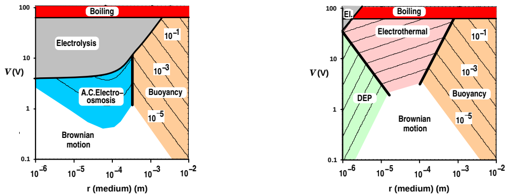
Figure 2. Particle velocity maps in the plane V versus r for a particle with radius a = 0.25\mu\text{m} in medium with \sigma = 10^{-1}\text{S/m} : (left) f = 10^4\text{ Hz} ; (right) f = 10^7\text{ Hz} .
