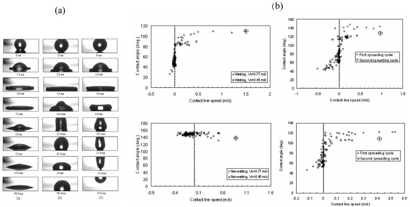
Figure 1. Sequence of time evolution of droplet impact on three different surfaces (a) and contact line speed dependence of the contact angle for all the surfaces studied (b).
