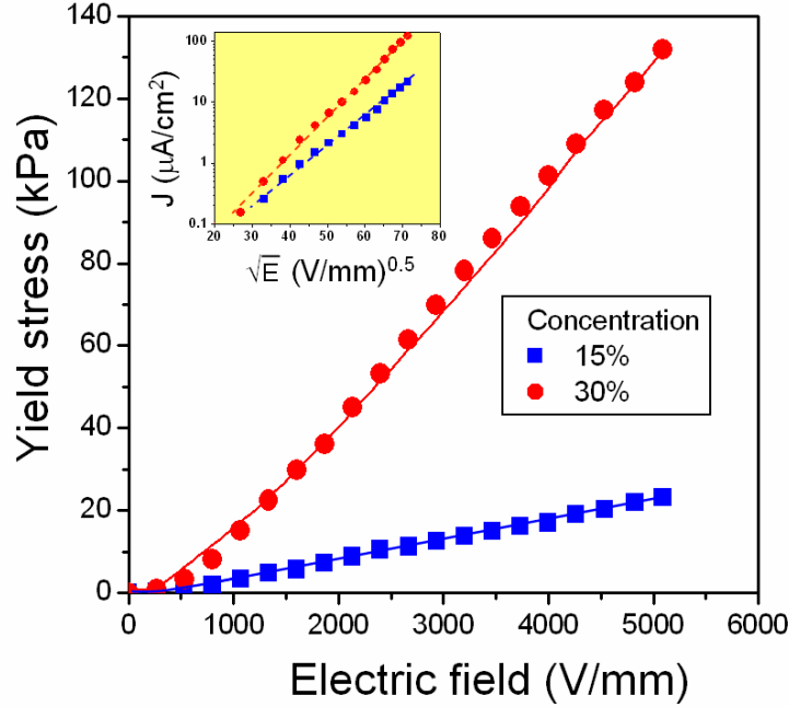
Figure 2 Static yield stress variation plotted as a function of applied electric field for two solid concentrations. Symbols denote experiment; solid lines are theory. Inset: logarithm of the current density J plotted as a function of \sqrt{E} . The dashed straight lines serve to delineate the \ln J \propto \sqrt{E} relationship, indicating the mechanism of activation over the Coulomb barrier [1].
