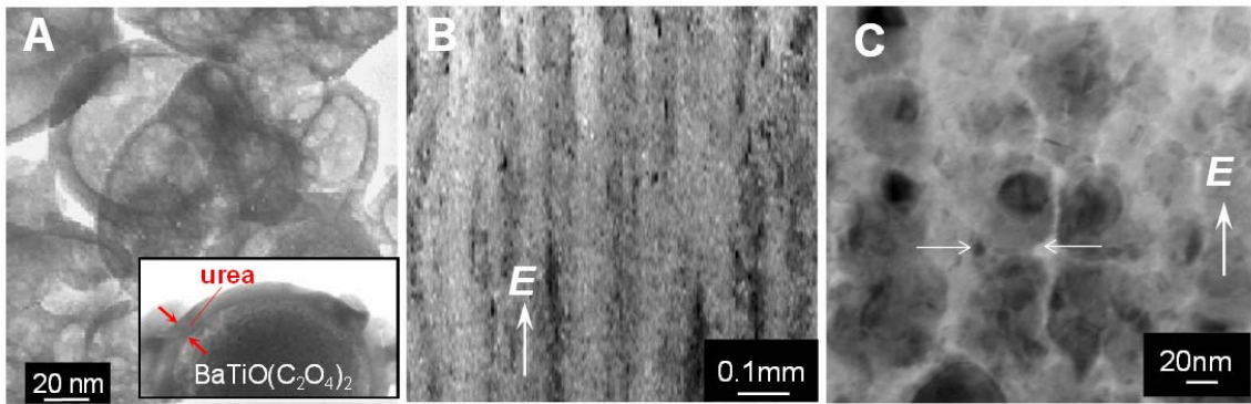
Figure 1 Images of nanoparticles in GER suspensions. (A) TEM image of coated nanoparticles. Urea coatings are clearly seen. (B) Optical microscope image of a sample prepared in epoxy, solidified under an applied field of 2000 V/mm. Aligned columns along the field direction are visible. (C) TEM image of a section of the column shown in (B). The arrows indicate one of the flattened interfaces [1].
