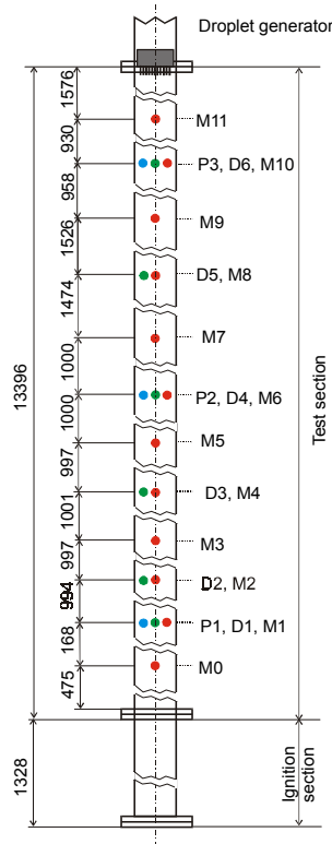
Fig. 1. Experimental setup
