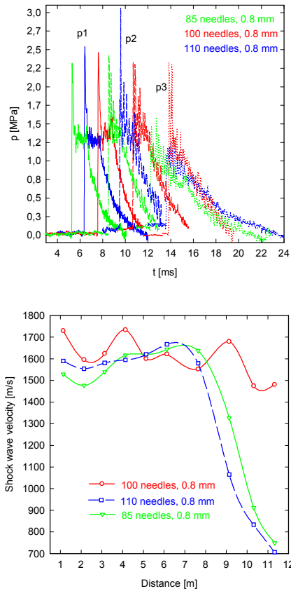
Fig. 2. Pressure profiles and shock wave velocities in hexane spray – air mixtures produced with 85-, 100- and 110-needle generators, pressure in the booster – 0.4 MPa
