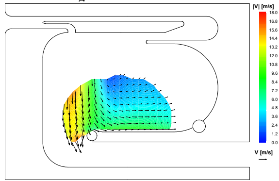
Figure 2. Effect of the Air 1 Flow Rate on the Mean Flow Structure
