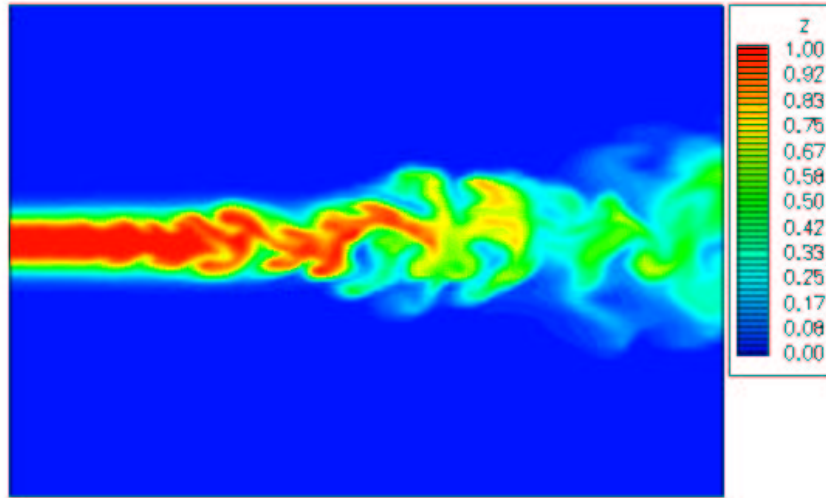
Figure 1. Mixture fraction contours in Sandia D flame.
