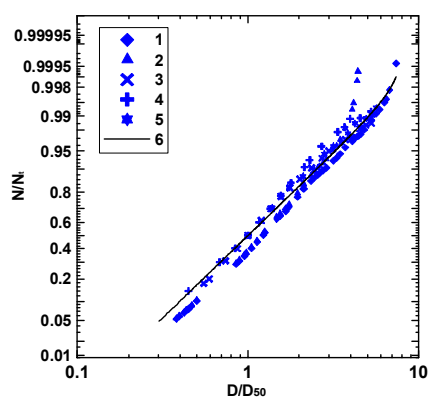
Fig. 5 Simulated (curve 6) vs. measured (1-5) self-similar size distribution of oil droplets.
