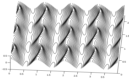
Figure 2. Free surface elevation of oscillating horse-shoe pattern.
