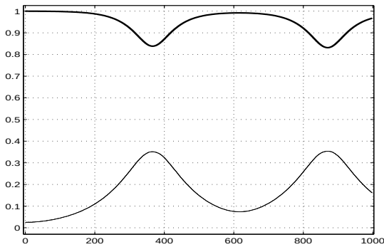
Figure 1. Typical energy evolution for the main modes corresponding to a recurrence cycle ( (ak)_0 = 0.13 ), fundamental (thick line) (k_0, 0) and perturbation (1.5k_0, q) .
