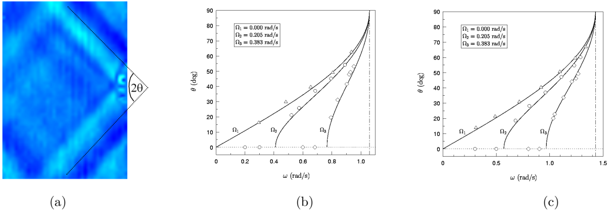
FIGURE 1 : (a) Cross section of a pair of conical wave beams originating from a sphere (center-right). N = 1.43 \text{ s}^{-1} , \Omega = 0.285 \text{ s}^{-1} , \omega = 1.11 \text{ s}^{-1} (b) Experimental results for N = 1.06 \text{ s}^{-1} (c) Experimental results for N = 1.43 \text{ s}^{-1} .
