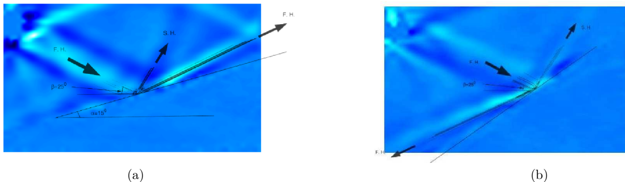
FIGURE 2 : Reflected internal wave beams. (a) \theta = 25^\circ, \phi = 15^\circ . (b) \theta = 25^\circ, \phi = 35^\circ .
