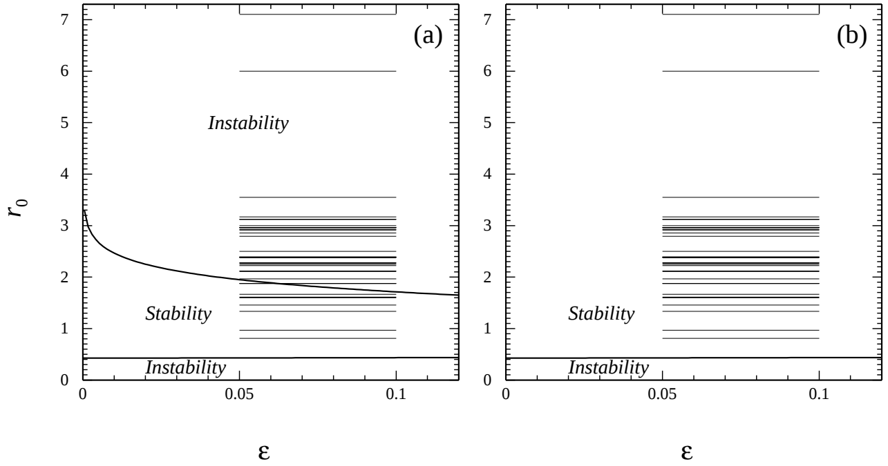
Figure 1. Stability of (a) compensated vortices, and (b) vortices with uniform PV in the lower layer, on the (\epsilon, r_0) -plane ( \epsilon is the depth ratio of the ocean, r_0 is the nondimensional radius of the vortex). Horizontal segments show the rings catalogued by Olson (1991).
