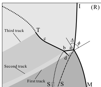
Fig. 3 The making of structural tracks in a numerical detonation cell
