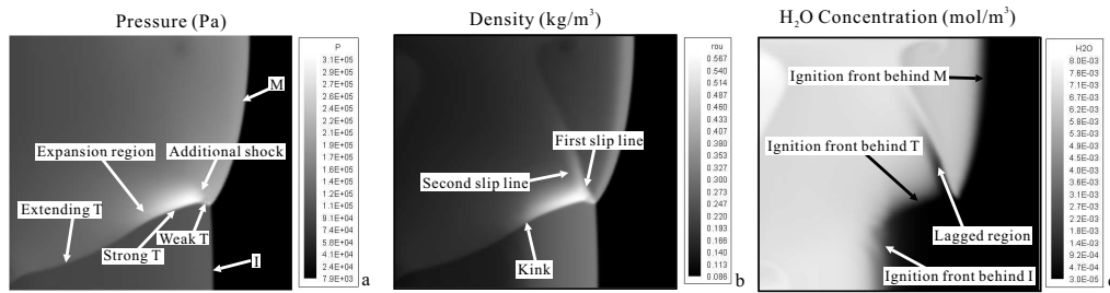
Fig. 1 Cellular structure with one transverse wave with 0.025mm grid size a)pressure, b)density, c)d)H 2 Oconcentration
