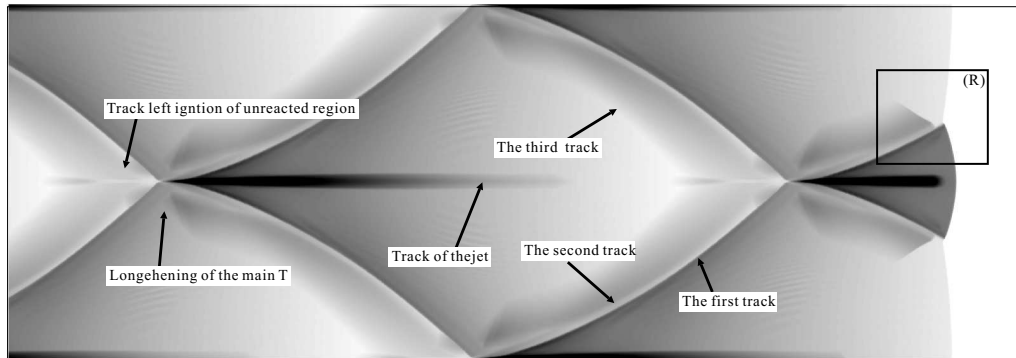
Fig. 2 Numerical detonation cells in a 8mm channel (region (R)) is produced schematically in Fig. 3
