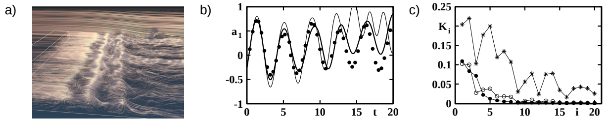
Figure 2. 20-dimensional Galerkin model of the transitional flow over a back-ward facing step at Re_h = 3000 . (a) Snapshot of the streamlines (the step is indicated by a white frame) [5]. (b) The Galerkin model with the turbulence representation (thick curve) follows the LES simulation (•) over on a longer time than the model without turbulence representation (thin curve). (c) Modal energy distribution K_i ( i being the mode index). The LES results (•) are significantly better predicted with the enhanced turbulence model (o) than without it (*).
