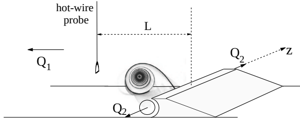
Figure 1. Experimental set-up.
