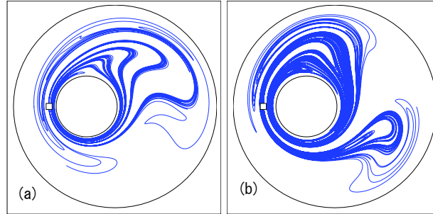
Fig.1 Stable manifolds of unstable fixed points denoted by squares. \alpha = 0.3 , \varepsilon = 0.4 . (a) T_o = 1.0 , T_i = 6.0 , (b) T_o = 0.5 , T_i = 3.0 .
