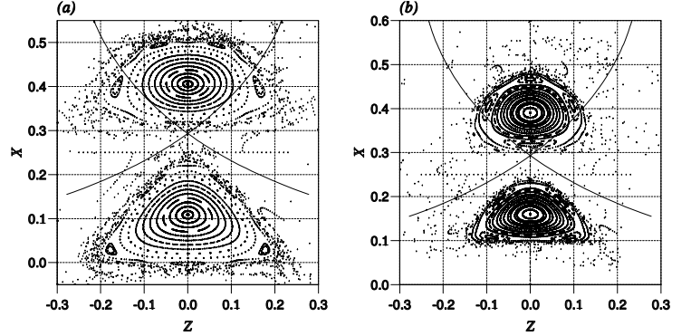
Figure 2. Poincaré sections for trajectories of (3) with various initial conditions. Poincaré plane is located at y = 0 . The parameter values are (\nu, \tau) = (1.924, 0.3827) and (a): G = 0.1832 , (b): G = 0.3113 .
