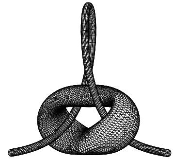
Figure 1. Torus with the vortex soliton.
