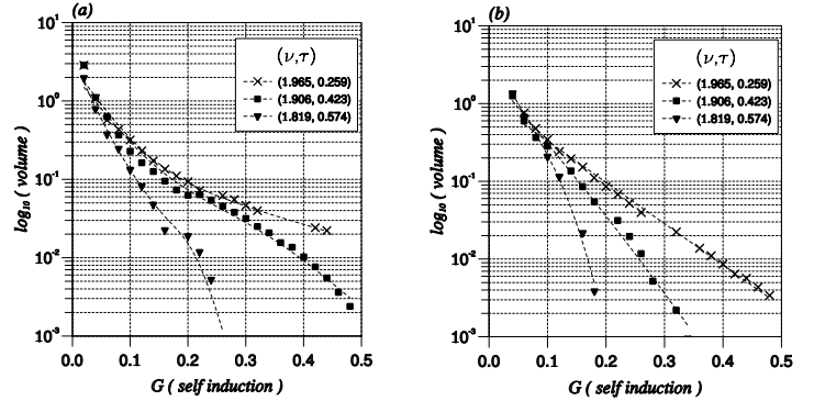
Figure 3. Comparison of the volume of the outmost torus as a function of G for three different combinations of \nu and \tau . (a) vortex soliton, (b) chopsticks model
