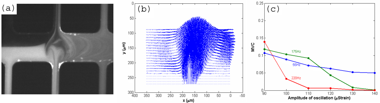
Figure 2: (a) flow visualization for large amplitude of oscillation and large frequency in the middle plane. (b) PIV measurement in the same configuration. (c) MVC for different frequencies and amplitudes.
