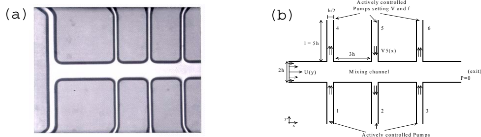
Figure 1. (a) micrograph of the mixing chip, (b) schematic showing one possible flow configuration.
