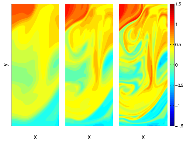
Figure 1. Slices of the total scalar field (mean plus fluctuation) for Sc = 1 (left), 8 (middle), and 64 (right), all of which are advected by the same flow. Only a fraction of the simulation domain is shown.
