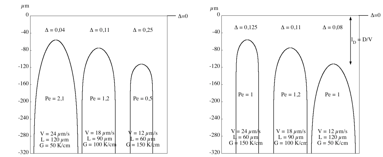
Fig 2 : Examples of cell geometries ranging from large sharp shapes to thin rounded shapes. Lines correspond to the shapes recovered by the fitted function with adequate parameters. The position of cell tips have been set so as to correspond to the undercooling relationship determined in [5], The Péclet number and the solutal diffusivity are denoted Pe = LV/D and D respectively.
