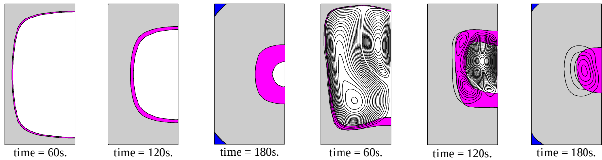
Fig.1. Solidification of Al 2 %wt_Cu in a sand mould: white – liquid phase, pink – under-cooled liquid zone, grey – mushy zone, dark blue- solid phase.
