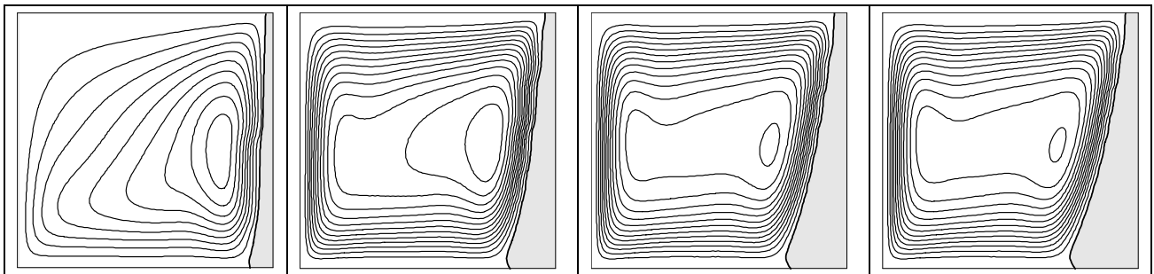
Fig.3 Enthalpy-porous medium model: the calculated flow pattern and solid phase shape after 100s, 500s, 1000s and 2000s (from left to right) of solidification of 3.5%wt aqueous solution of NH 4 Cl.
