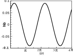
Figure 2. The interface position oscillates as a function of time.
