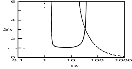
Figure 3. The neutral curves in terms of the Sekerka number S_k and the wave number \alpha . The left curve corresponds to the synchronous mode and the right curve the subharmonic mode.
