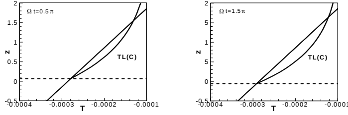
Figure 1. The instantaneous temperature T and melting temperature T_L at two phases of a period: (a) \Omega t = 0.5\pi , (b) \Omega t = 1.5\pi .
