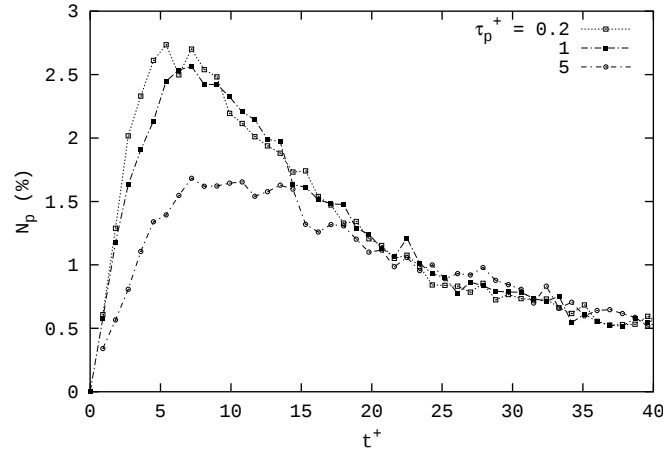
Figure 1: PDF of the time spent by the swept-and-reentrained particle in the viscous sublayer ( z^+ < 5 ).
