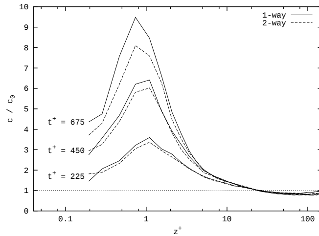
Figure 2: Time evolution of the \tau_p^+ = 5 particles number distribution profiles as a function of the wall normal direction.
