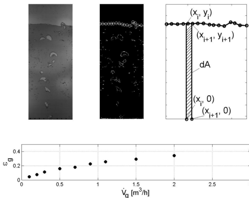
Fig.1. Volume fraction's determination method. This parameter is calculated strictly from the area of the two phase bed.
