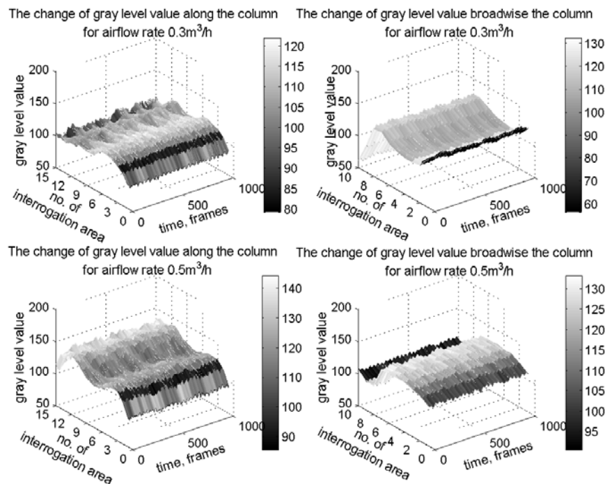
Fig. 3 The change of the gray level in time in airflow range 0.3 \div 0.5 \text{ m}^3/\text{h} . Diagrams on the left illustrates the change along the apparatus (interrogation area no. 1 – bottom, no. 15 – top of two-phase bed) and diagrams on the right illustrates the change broadwise the column (1 – left side, 10 – right side of the bed). 1000 frames = 9.7 s.
