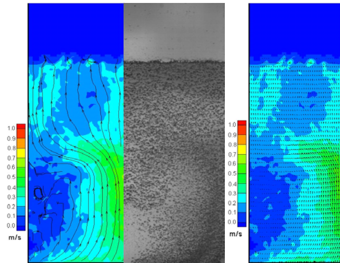
Fig.2 Velocity fields and bubbles' trajectories calculated for airflow rate 0.3 \text{ m}^3/\text{h}
