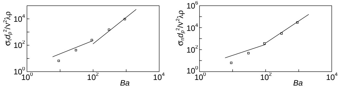
Figure 2. Non-dimensional shear (left) and normal (right) stress as a function of the Bagnold number ( Ba=St \cdot \lambda^{1/2} if \rho_s=\rho_l , with \lambda=1/[(\phi_0/\phi)^{1/3}-1] , and \phi_0=0.74 the closest packing of spheres volume fraction). The solid lines are the empirical correlations due to Bagnold [1], the symbols are simulation results for \phi=0.46 ( \lambda=5.8 ).
