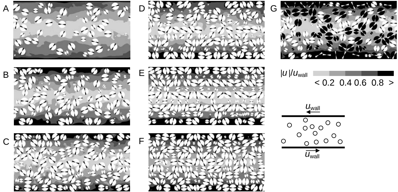
Figure 1. Cross-sections of single realizations of the solid-liquid flow. In cases A-F the particles have uniform size and St=375 ( St is defined in the text). The solids volume fractions in cases A-F are 0.26, 0.37, 0.46, 0.50, 0.55, and 0.59 respectively. Case G has the same solids volume fraction as case D, except that in case G there are two particle diameters: one 0.9 times (white), and one 1.1 times (black) the diameter of case D. The gray scale denotes the absolute value of the liquid velocity. The collisions are elastic and frictionless.
