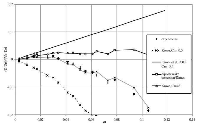
Figure 2 : Comparison between drift models and experimental results ( U_{cl} denotes U_{FF} )
