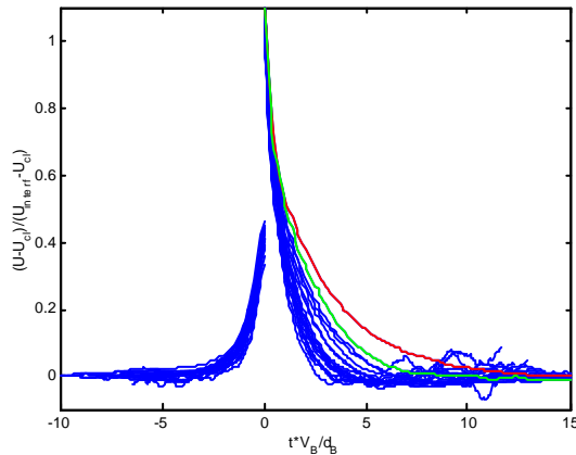
Figure 1 : Phase average of the velocity around the bubbles (red : minimum void fraction ; green, then blue : void fraction increases)
