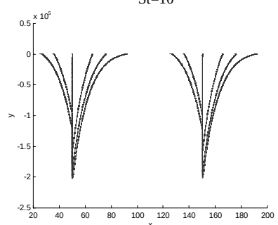
Figure 3: trajectories of inertial particles with neighbouring vortices swirling anticyclonically for small or moderate particle inertia.
