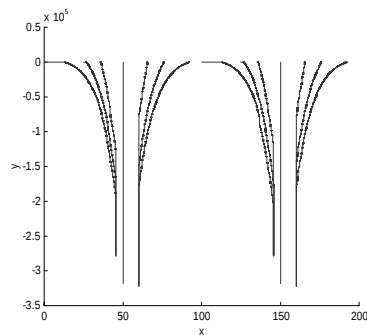
Figure 4: trajectories of inertial particles with neighbouring vortices swirling anticyclonically for large particle inertia.
