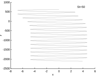
Figure 1: trajectories of inertial particles with neighbouring vortices swirling alternatively cyclonically and anticyclonically for small particle inertia.
