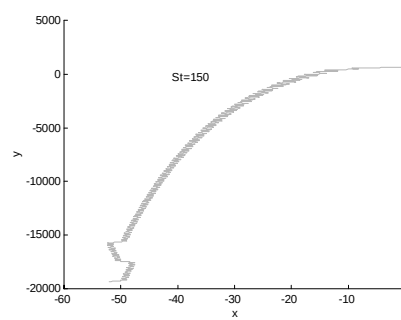
Figure 2: trajectories of inertial particles with neighbouring vortices swirling alternatively cyclonically and anticyclonically for moderate particle inertia.
