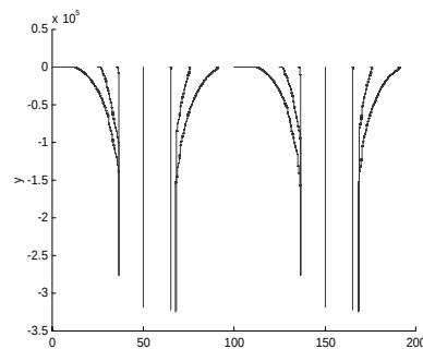
Figure 4: trajectories of inertial particles with neighbouring vortices swirling anticyclonically for large particle inertia.
