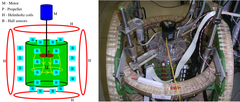
Figure 1. Schematic view (left) and laboratory set-up (right) of the CIFT experiment. The propeller driven flow of a metallic melt is exposed alternately to a transverse and an axial magnetic field, which are produced by two pairs of Helmholtz coils. The respective induced magnetic fields are measured at 49 Hall sensors.
