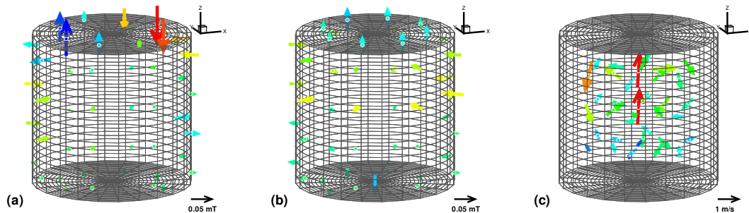
Figure 2. The measured induced magnetic fields for transverse (a) and axial (b) imposed magnetic field. The direction of the arrows indicates the measured field component. The reconstructed velocity field is shown in (c), where the colour indicates the flow speed.
