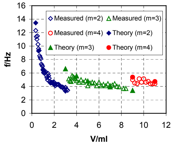
FIG. 3. Comparison between theory and measurement of the drop oscillation frequency.
