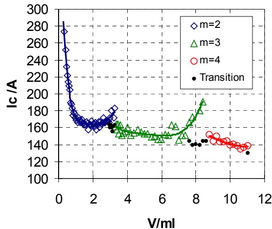
FIG. 2. Stability diagram of a puddle of GaInSn by 20kHz. Critical current for instability.
