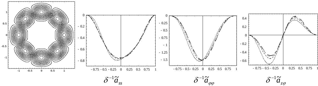
Fig.2. The functions \delta^{-1} \tilde{a} versus (s-1)/\delta for \delta m = \pi/2 and m=1, 2, 4, 16
