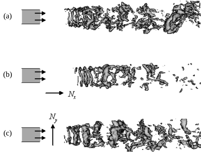
Figure 2. Instantaneous vortical structures: (a) without magnetic field; (b) N_x = 0.5 ; (c) N_y = 0.05 .
