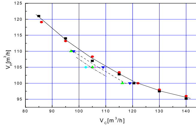
Figure 2: State diagram for dynamo action; steady state flow conditions ( \square pressure loss criterion; \bullet energy criterion, - fitting curve); periodic axial flow rates of period \tau = 7.5 s and a 5% change in amplitude ( \blacktriangledown pressure loss criterion, \blacktriangle energy criterion, --- fitting curve); periodic axial flow rates of period \tau = 20 s and a 10% change in amplitude (+ pressure criterion, \blacklozenge energy criterion, - • - • - conjectured fitted marginal line for dynamo action).
