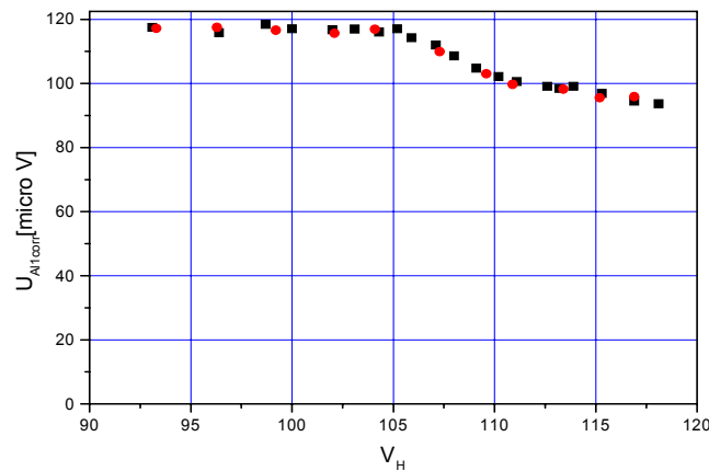
Figure 1: The measured compensated voltage at the Permanent Magnet Potential Probe located in an axial channel near the centre of the test module. One micro Volt (1 micro V) corresponds to a velocity of 0.04 m/s.
