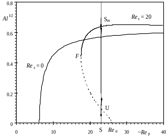
Figure 2. Bifurcation of magnetic field in a vortex-accretion flow.
