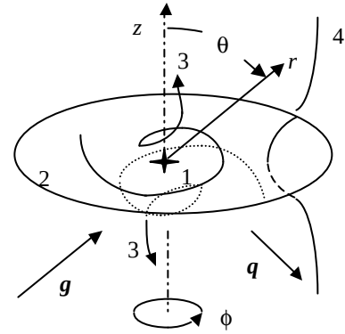
Figure 1. Schematic of a flow near a point source 1 of gravity \mathbf{g} and heat flux \mathbf{q} with accretion plane 2. Typical stream 3 and magnetic 4 lines are shown.
