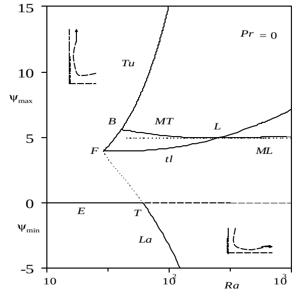
Figure 3. Bifurcations in a buoyancy flow.
