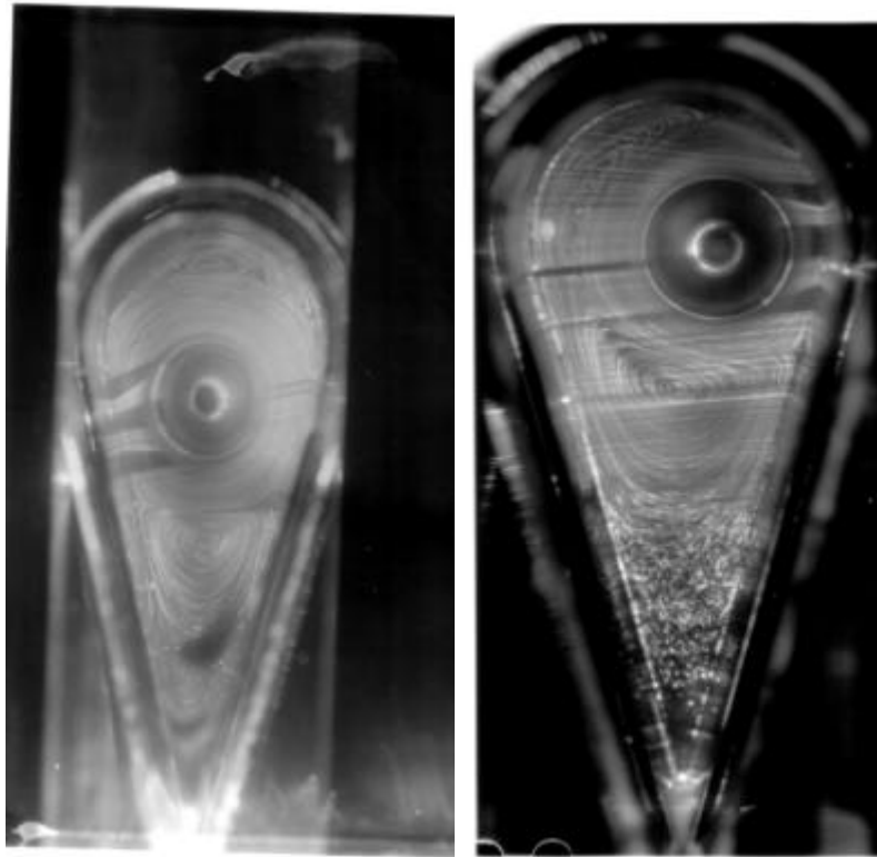
Figure 2- The visualization photographs for different positions of the cylinder.
