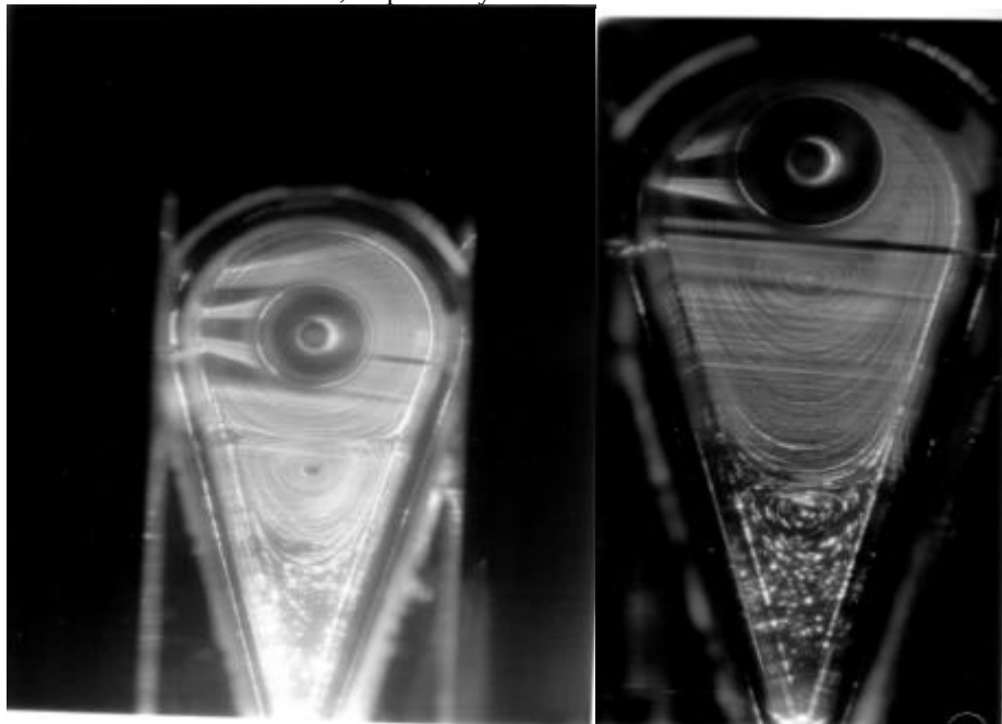
Figure 1- The visualization photographs for the exposure time of 15 (left) and 90 (right) minutes.
