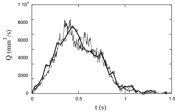
Figure 3. Time evolution of the avalanche flow rate Q based either on velocity profile ( Q_u , thin continuous line) or on the time decrease of the macroscopic pile angle ( Q_\theta , thick line).
