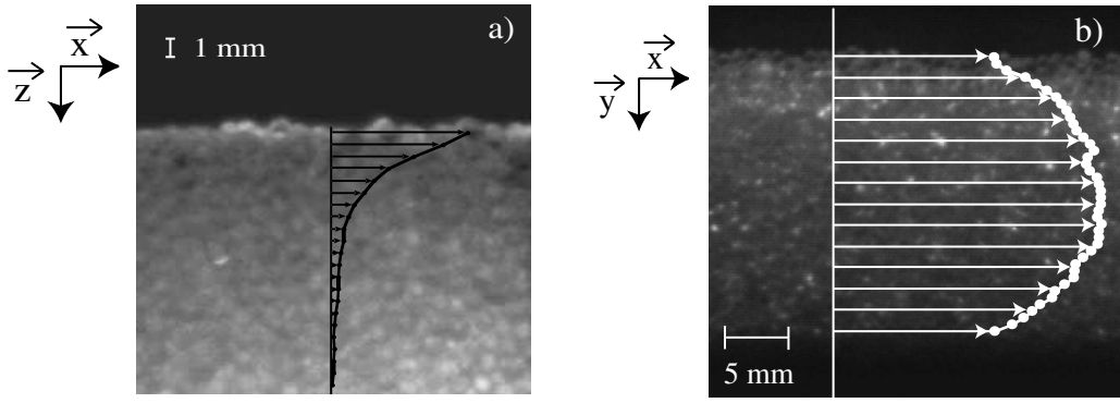
Figure 2. Images of the pile and corresponding instantaneous velocity profiles during an avalanche. (a) From the side at the front wall, (b) from above in between the walls.
