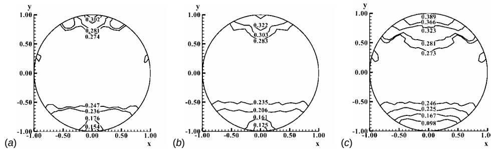
Figure 1. Contour plots of the concentration profile at 9.8 m downstream of the inline mixer for \phi_b = 0.20 and for experimental buoyancy numbers. (a) N_b = -2.1 ; (b) N_b = -4.2 ; (c) N_b = -8.7 .
