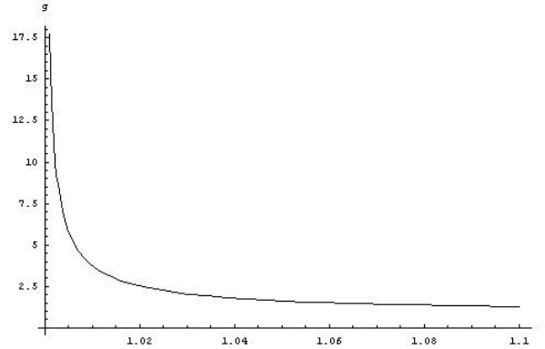
Figure 1. The two-particle reduced distribution function g(R) satisfying the finite correlation length criterion
