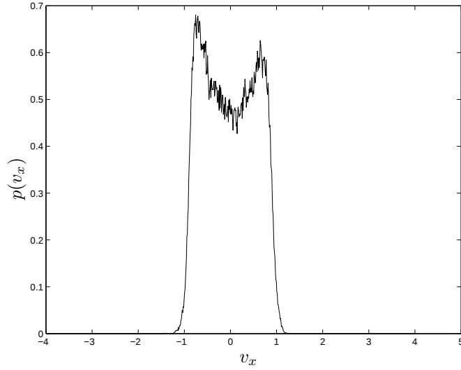
Figure 1. The probability density of the velocity in the x direction for a suspension of active particles of 10% area fraction.
