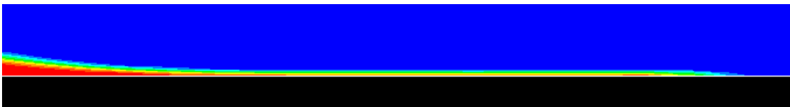
Figure 3: Liquid fraction contour of the residual liquid film left behind the liquid jet (Colour contours: liquid fraction = 1 (red), = 0.5 (green) = 0.0 (blue))
