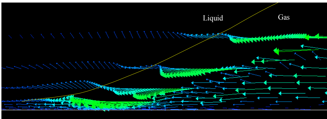
Figure 4: Velocity Vectors for liquid and gas jet system under normal operating conditions (Colour contours: velocity = 200 m/s (green), = 30 m/s (blue))
