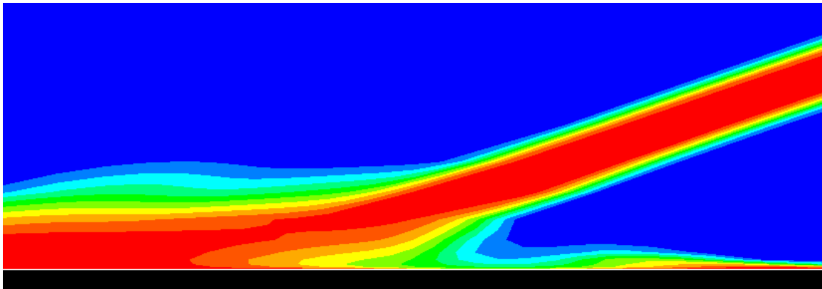
Figure 2: Magnified view of liquid jet with gas jet interaction under normal operating conditions (Colour contours: liquid fraction = 1 (red), = 0.5 (green) = 0.0 (blue))
