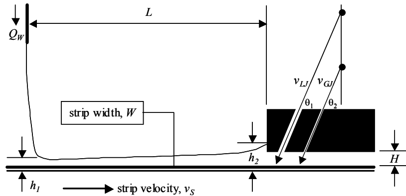
Figure 1: Basic Geometry for the Analytical Model
