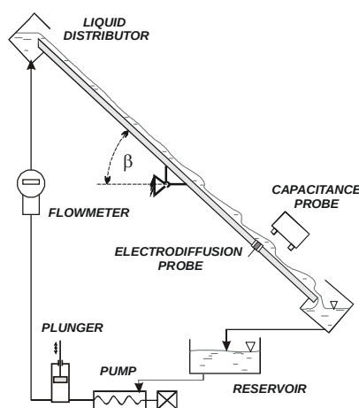
Fig.1 Experimental set-up
