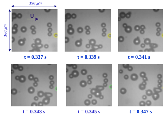
Fig.3 Visualization of the flow in the near-wall region just in front of the solitary wave.
