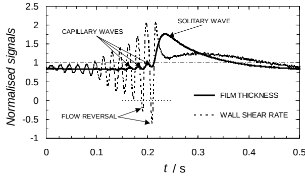
Fig.2 Film thickness and wall shear rate typical for the solitary wave regime (water data measured at f_p=1.8 Hz, Re=91 , \beta=6.5^\circ , x=1.5 m, h=0.63 mm, s=635 s ^{-1} , c=0.28 m/s).
