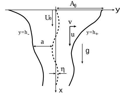
Fig.1 Schematic of a falling liquid sheet.
