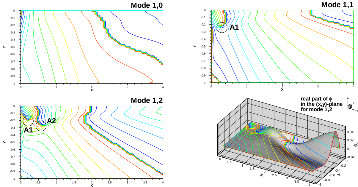
Figure 3. Phase of the eigenfunctions \phi for modes (1,0), (1,1), (1,2). The number of amphidromic points, Ai , depends on the frequency of the perturbation. The last graphic represents \phi_r that is oscillating and growing in x .
