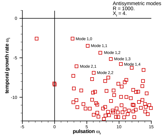
Figure 2. Part of the spectrum of the Taylor/Culick flow for the antisymmetric modes.
