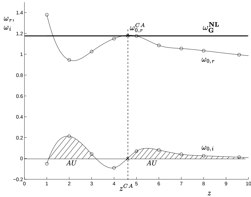
Figure 3. Streamwise evolution of the real \omega_{0,r} and imaginary part \omega_{0,i} of the local absolute frequency as a function of streamwise distance z .
