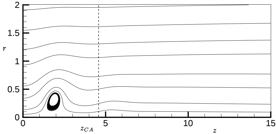
Figure 1. Meridional cut of the streamlines associated to the base flow obtained numerically by imposing the axisymmetry of the flow; S = 1.095 , Re = 200 (Ruith et al. [5]).
