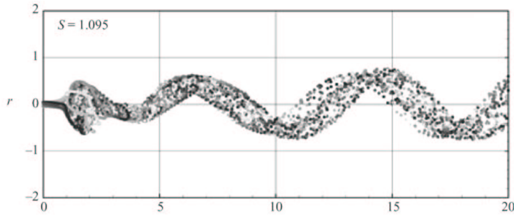
Figure 2. Instantaneous streaklines at t = 1850 associated to the three-dimensional flow obtained by DNS at S = 1.095 and Re = 200 (Ruith et al. [5]).
