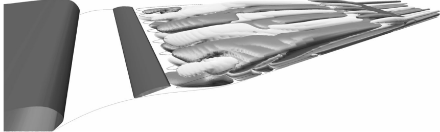
Figure 4: Isosurfaces of \omega_x = \pm \text{const.} ; grey : \omega_x > 0 ; white: \omega_x < 0 . Black: regions subject to centrifugal instability with R < 0 .
