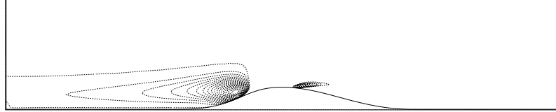
Figure 3: Isolines of negative R(x, u) -values indicating regions of possible centrifugal instability.
