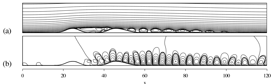
Figure 1: Instantaneous streamlines of (a) the total flow field and (b) the perturbation u' , at Re = 900 .
