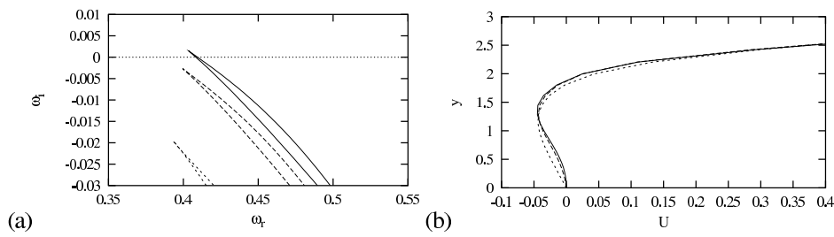
Figure 2:(a) Imaginary part \omega_i of complex frequency at the cusp \frac{\partial \omega}{\partial \alpha}(\alpha_0) = 0 as function of \omega_r and (b) the corresponding profiles, at x = 33 ; ...: Re = 600 , - - -: Re = 850 , —: Re = 900 .
