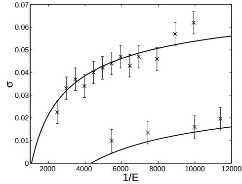
Figure 2. Growth rate versus the inverse of the Ekman number for \varepsilon = 0.08 (lower) and \varepsilon = 0.16 (upper). Experimental results ( \times ) and linear theory (solid line).
