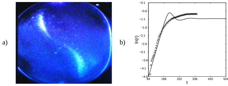
Figure 1. a) Visualisation of the spin-over mode in a meridional plane. b) Comparison between the experimental results ( \times ) and the nonlinear model. ( E = 2.5 \cdot 10^{-4} and \varepsilon = 0.16 ).
