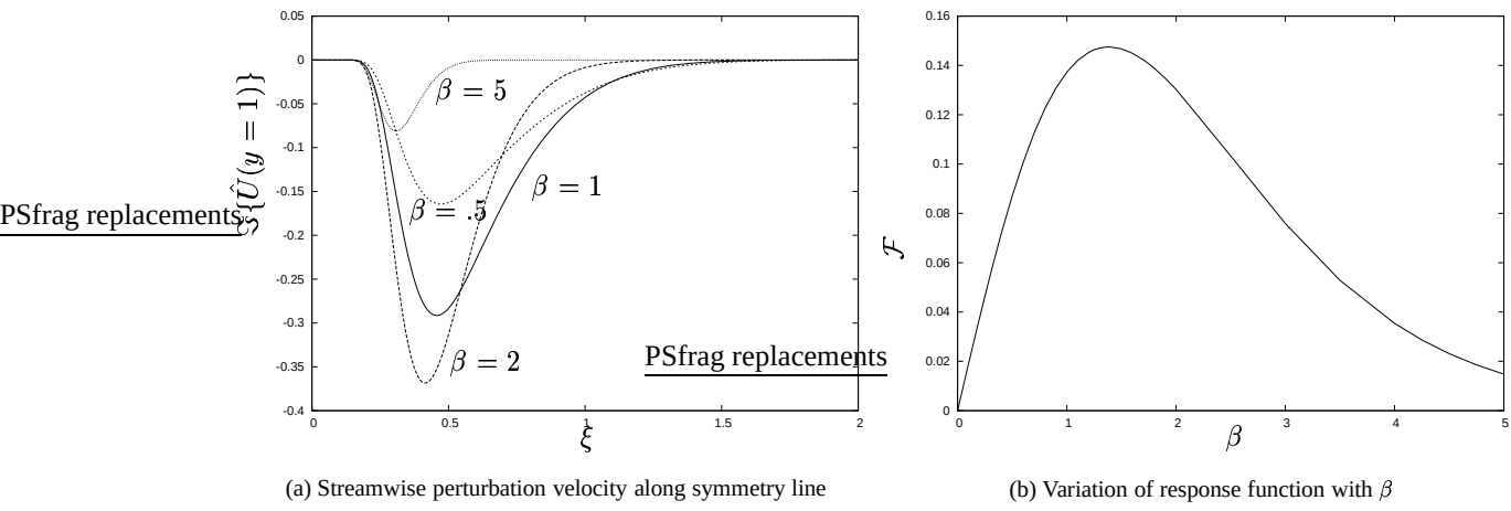
Figure 1. Channel results ( \omega = 0 )
